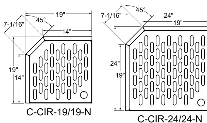
PLAN VIEWS
